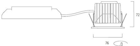
Dimensions (mm)
